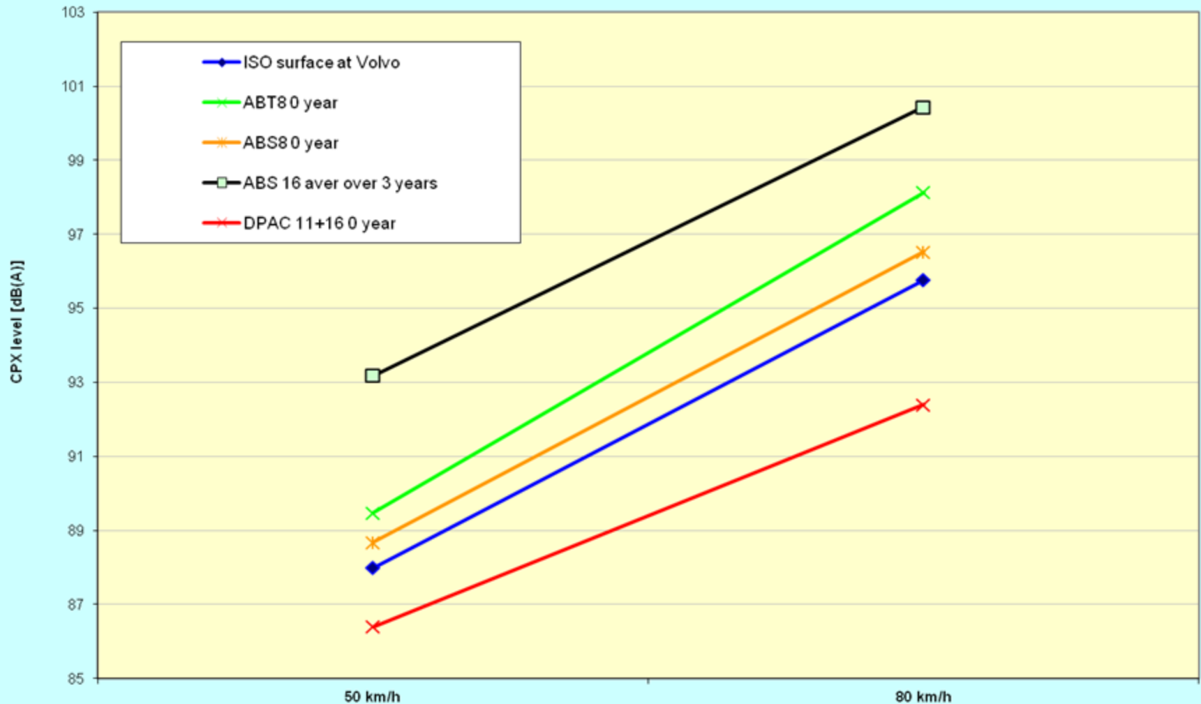
Comparison of Volvo ISO track with real road surfaces - AAV4
