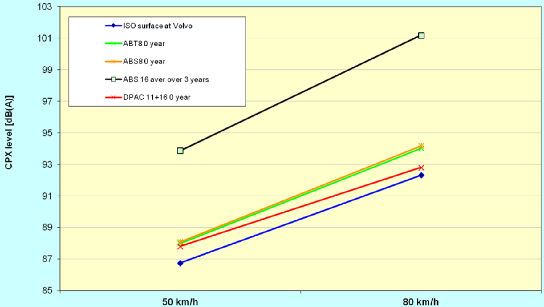
Comparison of Volvo ISO track with real road surfaces - SRTT
