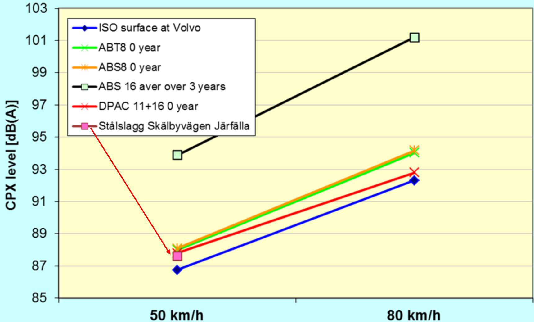
Comparison of Volvo ISO track with real road surfaces - SRTT
